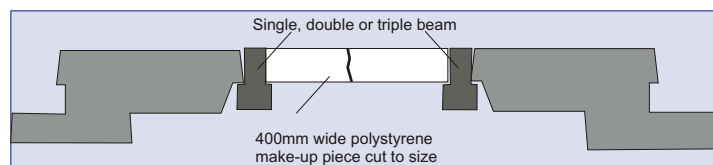
Section Y-Y
