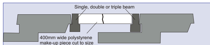
Section Q-Q
