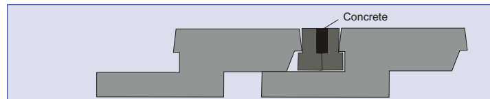
Section G-G
