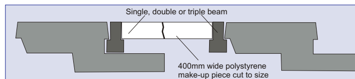
Section T-T
