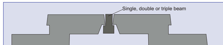
Section X-X
